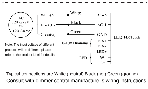
Wiring diagram
